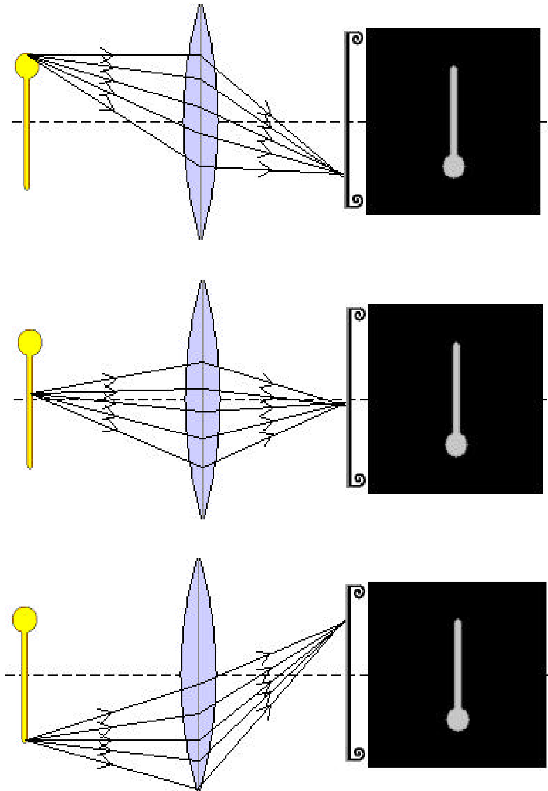
Figure 17. Three screen shots from the lens simulator, showing a spray of light rays leaving three different points on the source. As the spray
