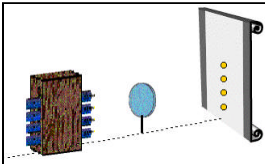
Figure 15: Set-up with four maglite point sources mounted vertically above one another, a converging lens and a screen. The four point images correspond to the four point sources.
