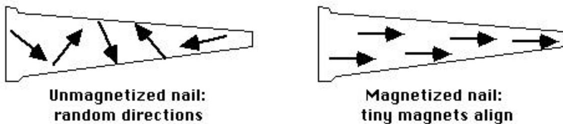
Figure 4. A formal model of magnetism. Arrows represent microscopic magnetic domains within the nail.
