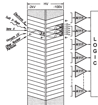
A Microchannel Plate (MCP) Array Connected to Multiple A111s
